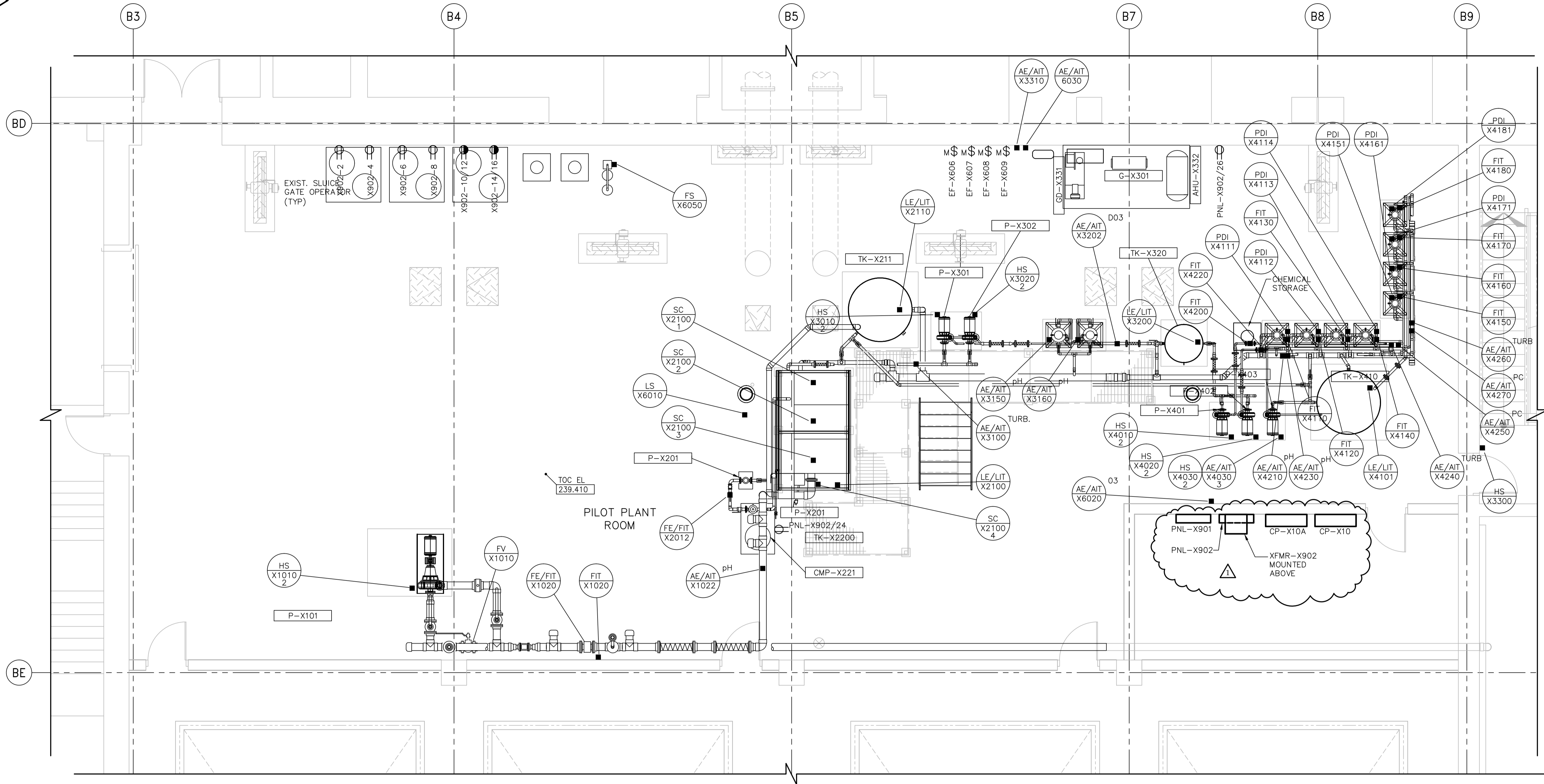
1 PILOT PLANT PLAN 1:50
